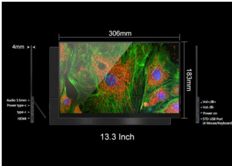
Dimension, Interface and Control Button of MD1080P1330 Displayer
