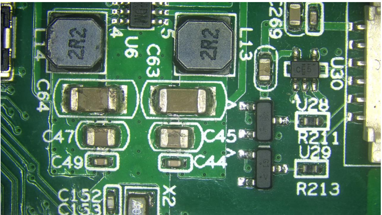
Figure 33 Circuit Board Captured with SVPRO4KUHD8MP
