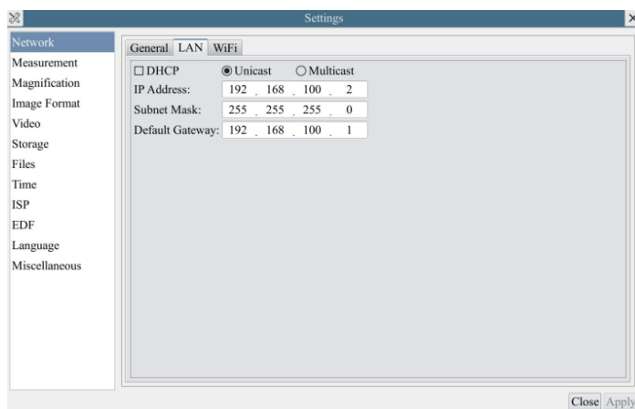
Figure 16 Configure the UPROAF4KUHD16MPCA_EF Camera IP
