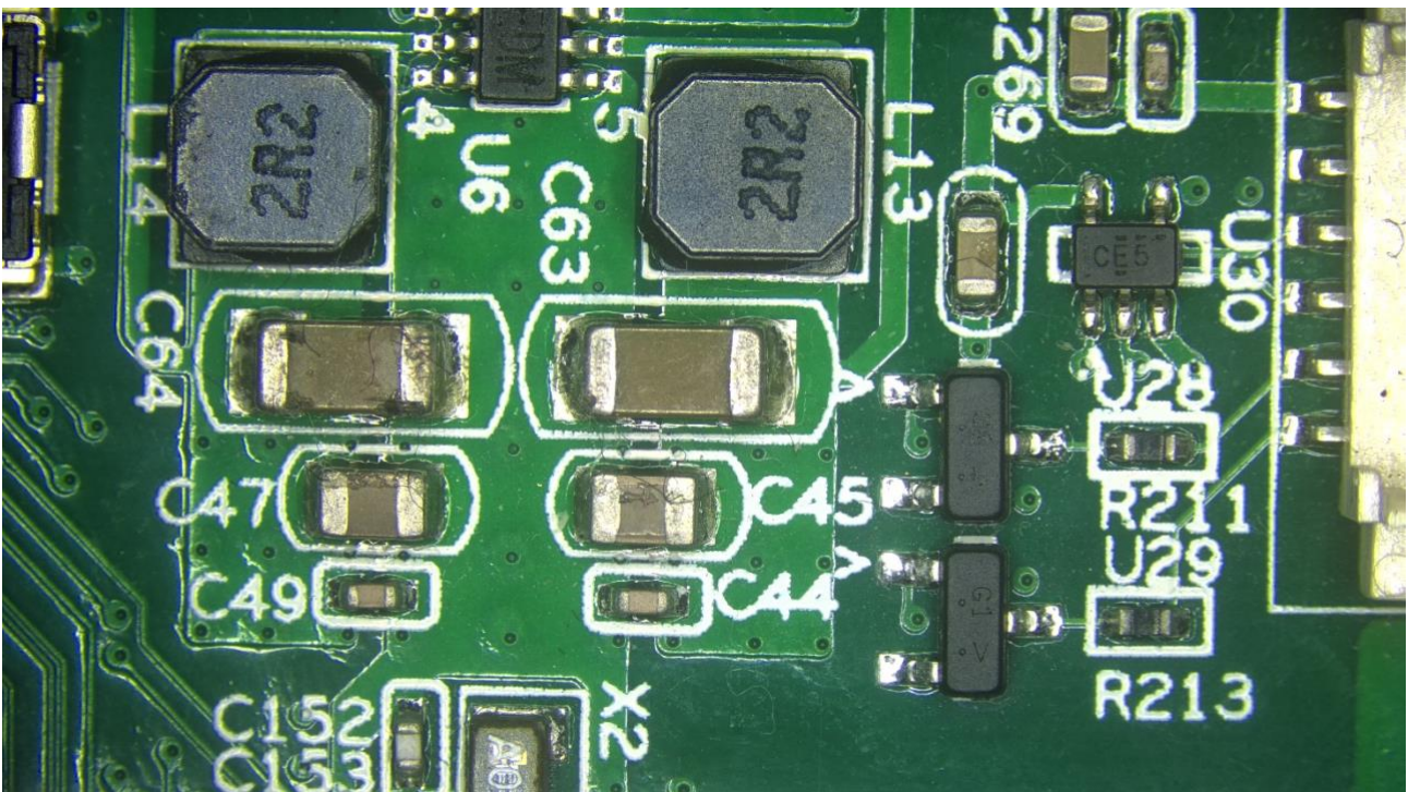
Figure 29 Circuit Board Captured with SVFL4KUHD8MPCA
