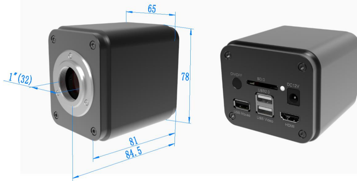
Figure 3 Dimension of SVFL4KUHD8MPCA
