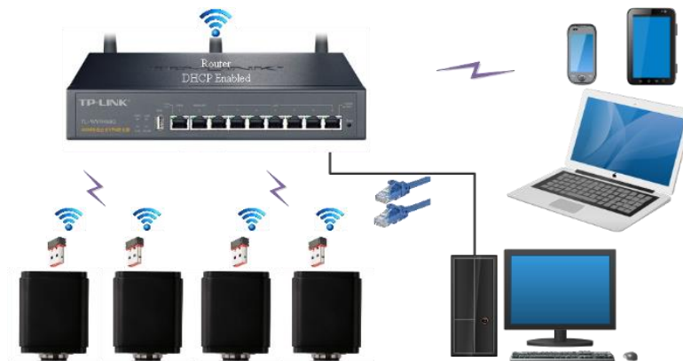
Figure 10 Multi SVFL4KUHD8MPCA Cameras Connecting to the Router through the WLAN Style
